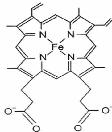
Figure 4: Structure of Tetra Pyrrole Head of Hemoglobin
