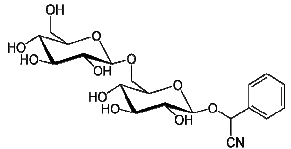
Figure 2: Structure of Laetrile
